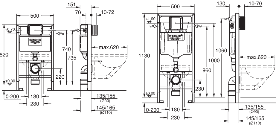
Rapid SL 0.82m Installation Height 38 526 000
