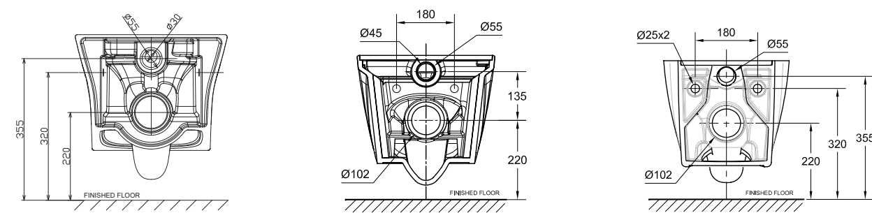
Signature Wall Hung WC CCAS3140-3W20400FO + CCASC119-U20U420CO
